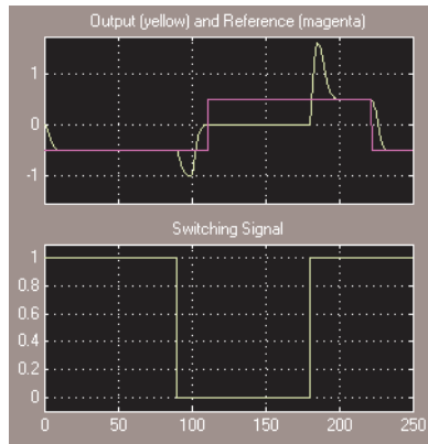
Figure 4-34: Output Response with Manipulated Variable Feedback Disconnected
