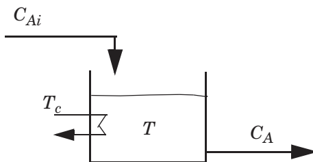
Figure 1-3: CSTR Schematic
