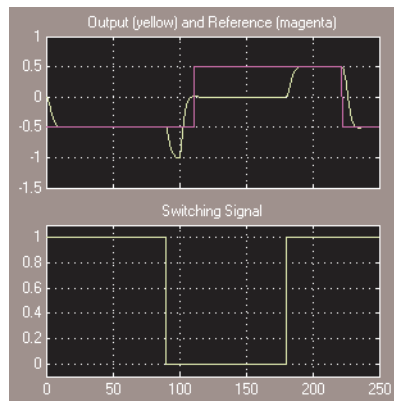
Figure 4-31: Output, Reference and Switching Signal
