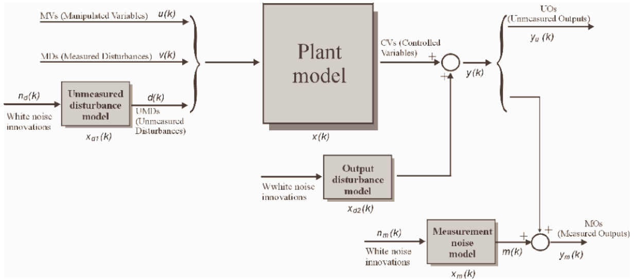
Figure 2-2: Model Used for State Estimation
