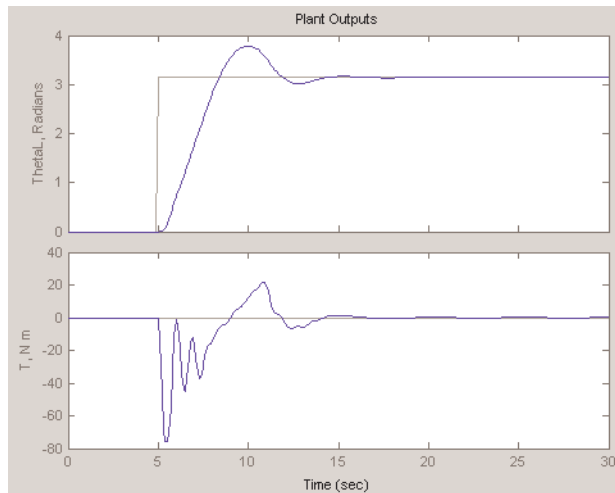
Figure 4-11: Servo Response for Step Increase of \pi Radians
